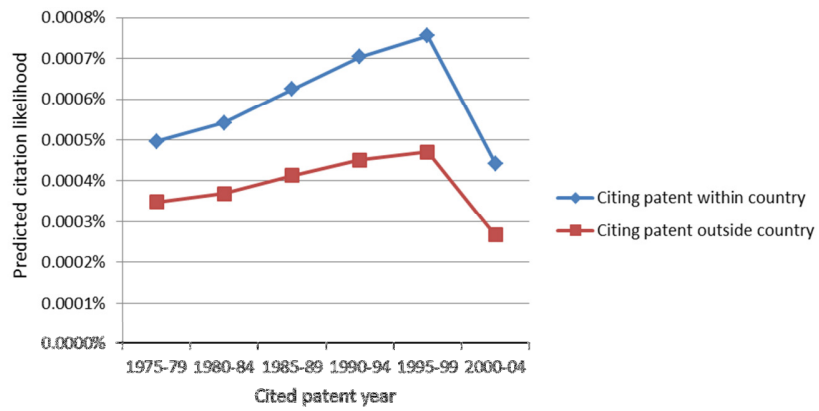
Figure 2. Predicted probabilities across different time periods
